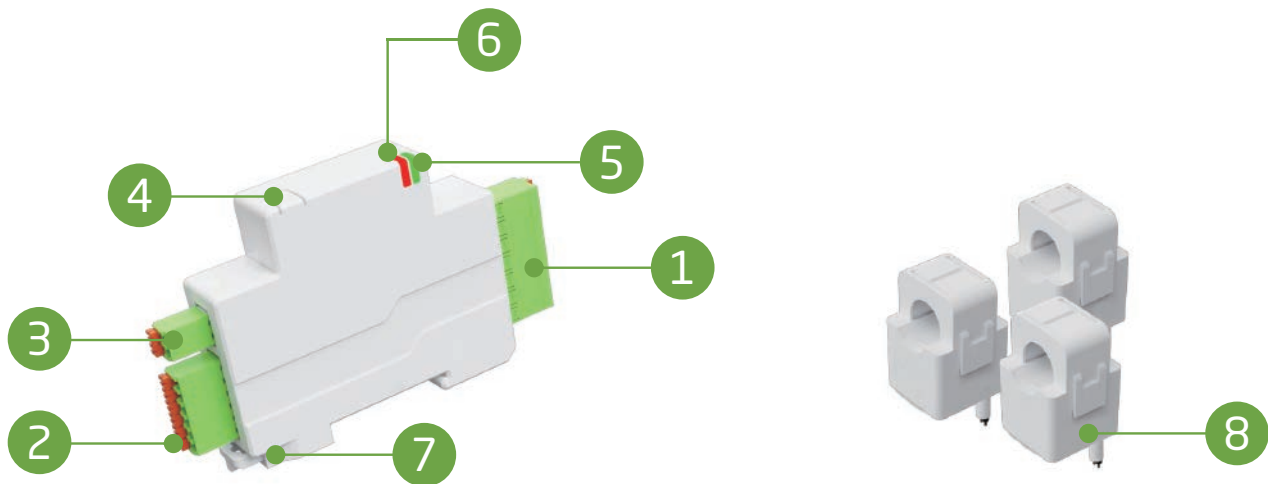
BPM3500 Energy Monitoring Module with Split core CT
